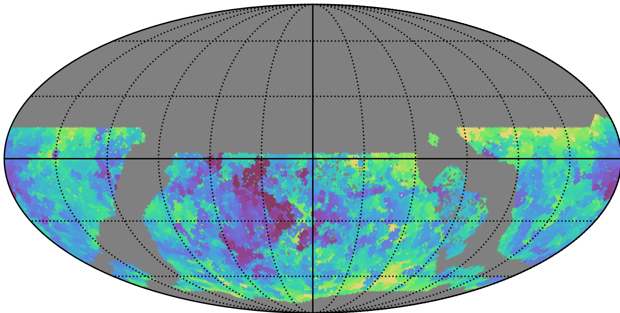
extra_ss_neo7_v3.4_10yrs WFD g band: Min seeingEff
