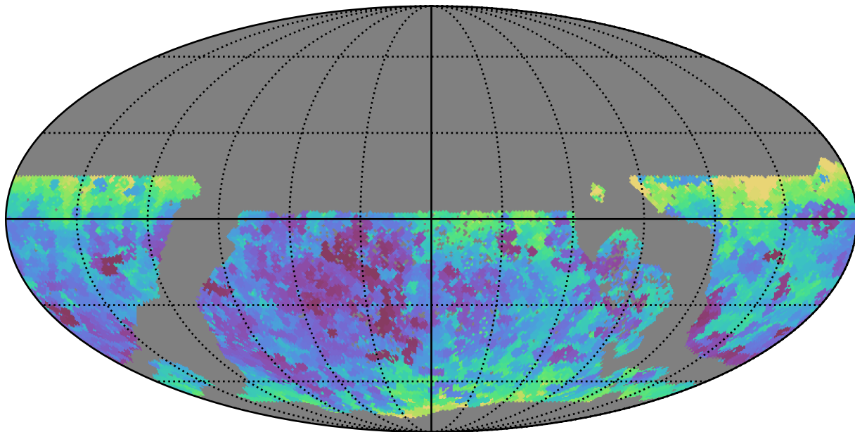
extra_ss_neo7_v3.4_10yrs WFD all bands: Min seeingEff
