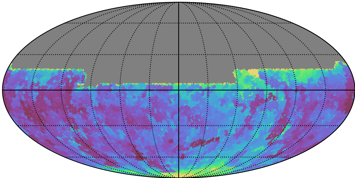
extra_ss_neo7_v3.4_10yrs All sky u band: Min seeingEff
