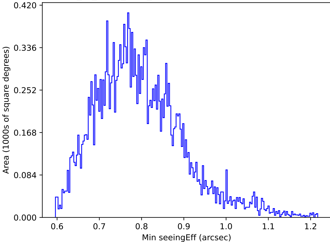
extra_ss_neo7_v3.4_10yrs All sky u band: Min seeingEff
