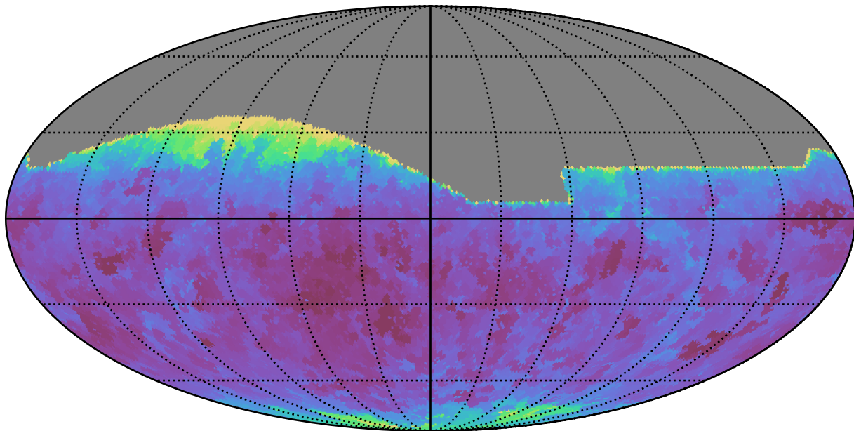
extra_ss_neo7_v3.4_10yrs All sky r band: Min seeingEff
