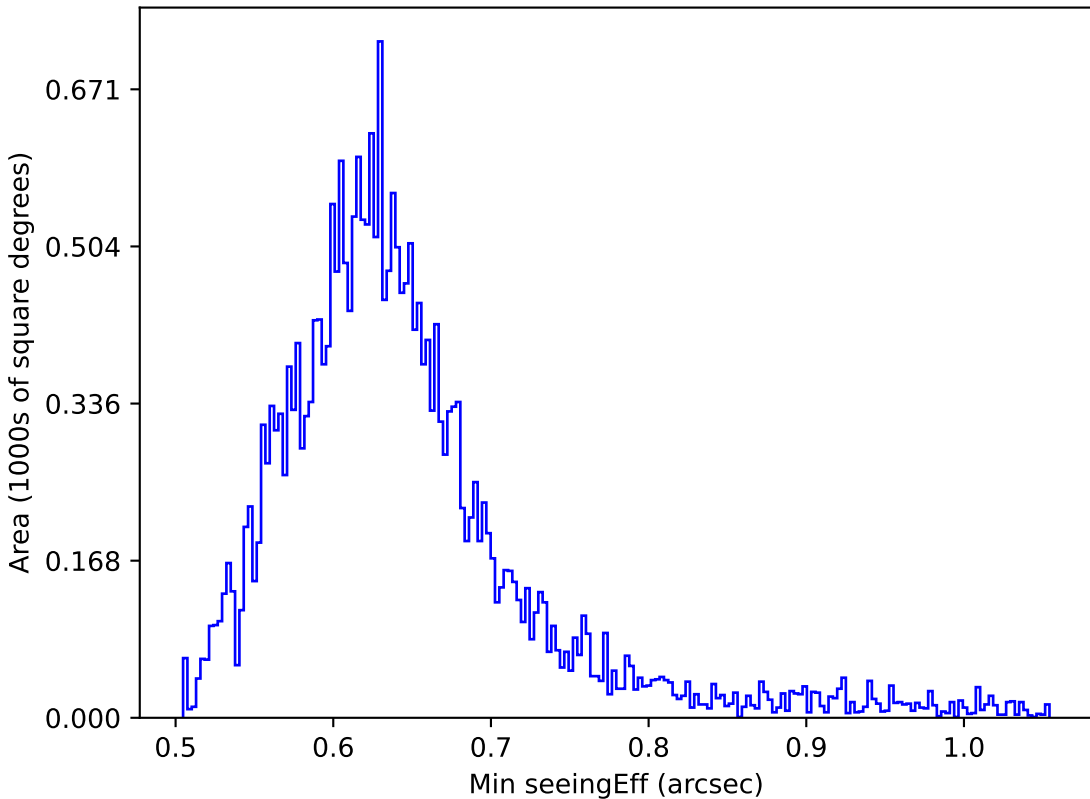
extra_ss_neo7_v3.4_10yrs All sky r band: Min seeingEff
