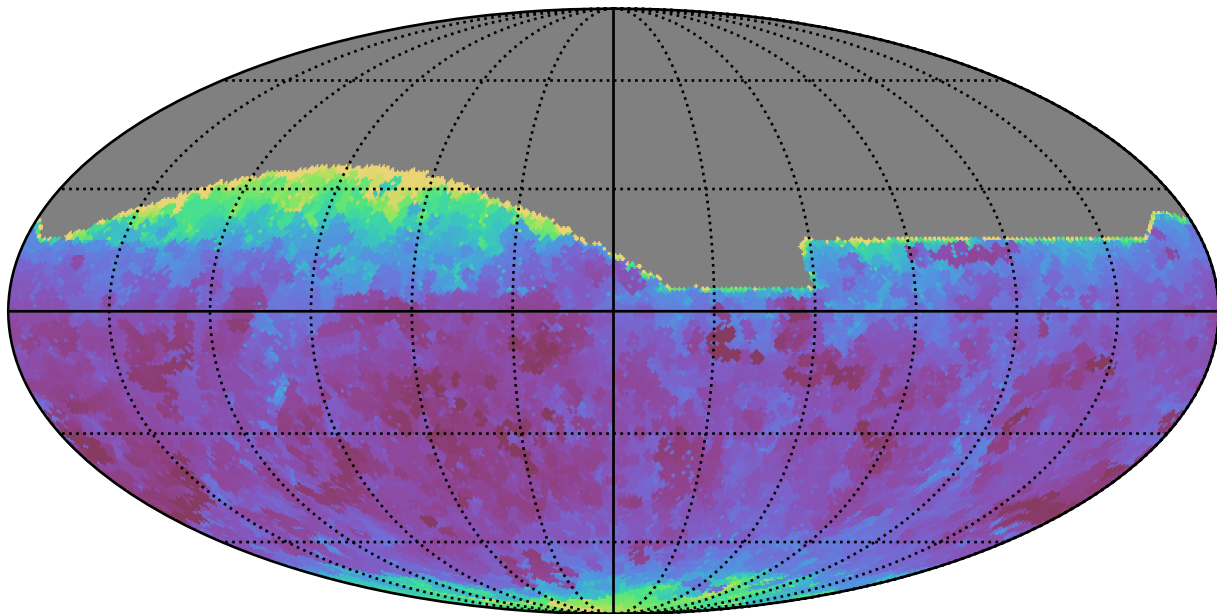
extra_ss_neo7_v3.4_10yrs All sky i band: Min seeingEff
