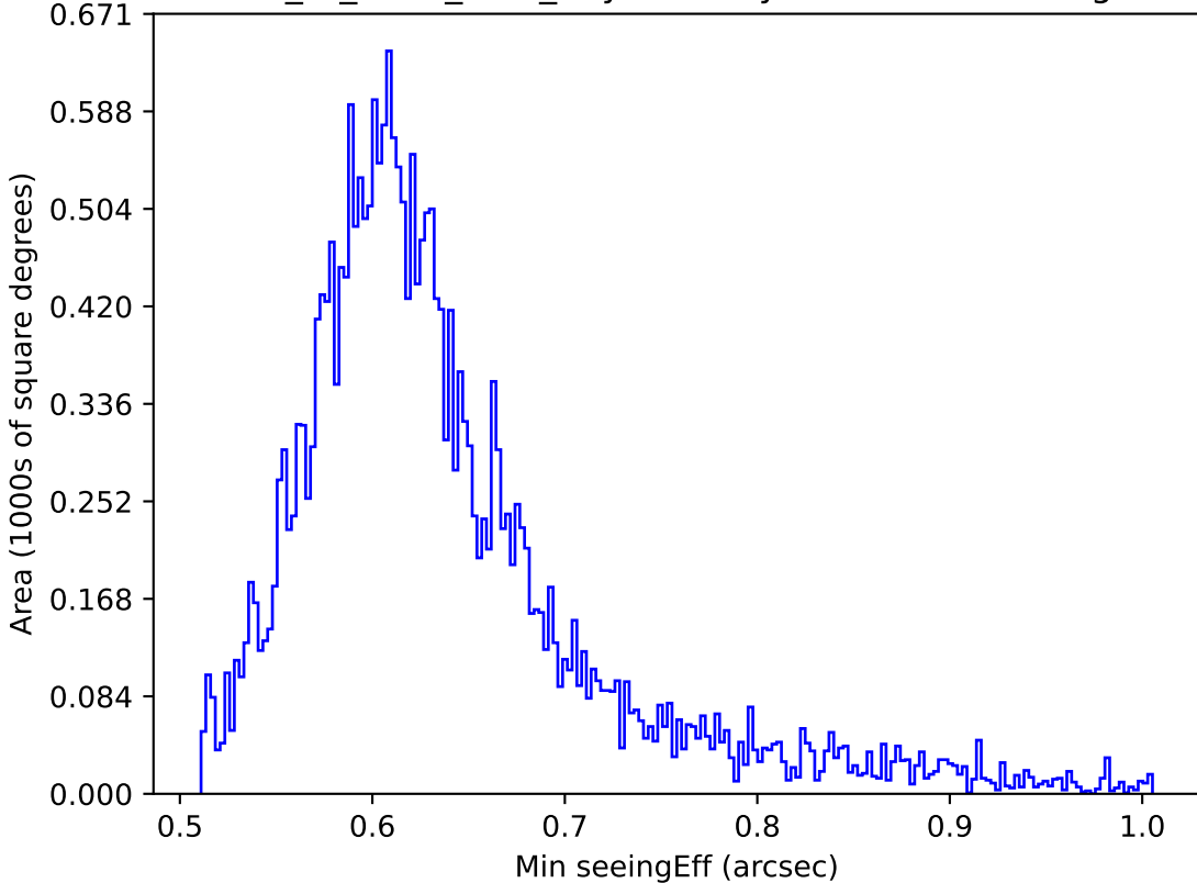
extra_ss_neo7_v3.4_10yrs All sky i band: Min seeingEff
