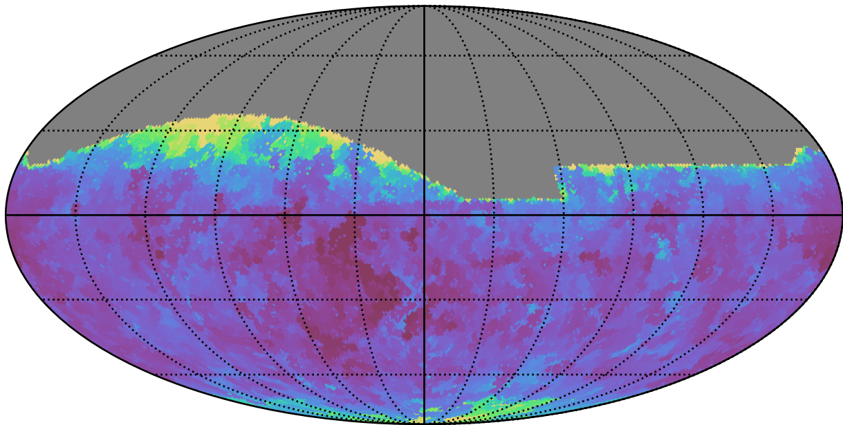
extra_ss_neo7_v3.4_10yrs All sky g band: Min seeingEff
