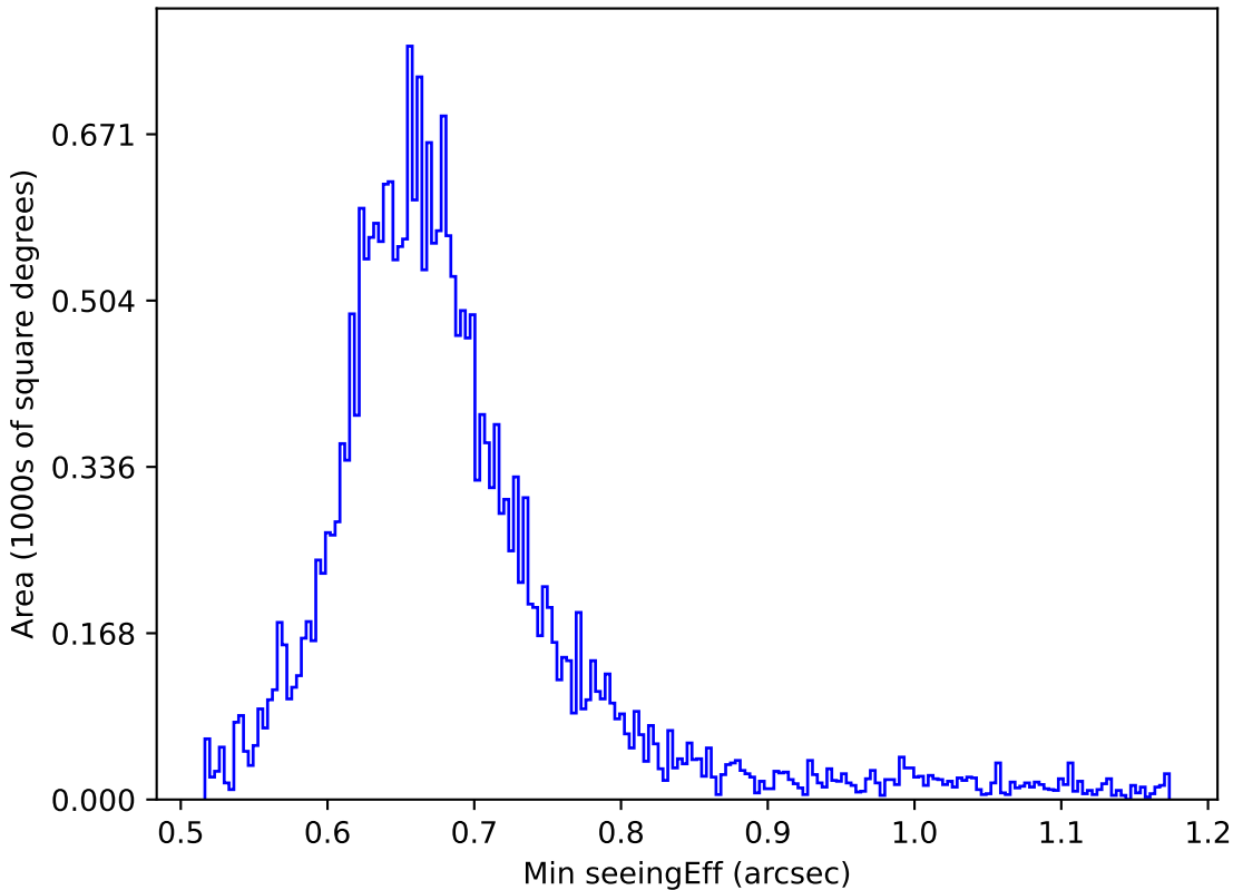
extra_ss_neo7_v3.4_10yrs All sky g band: Min seeingEff
