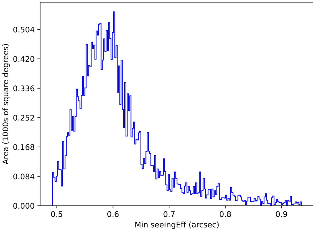
extra_ss_neo7_v3.4_10yrs All sky all bands: Min seeingEff
