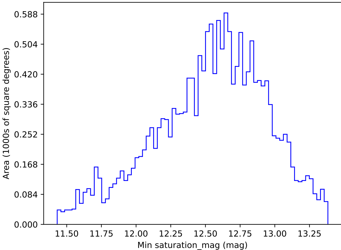
extra_ss_neo7_v3.4_10yrs WFD r band: Min saturation_mag
