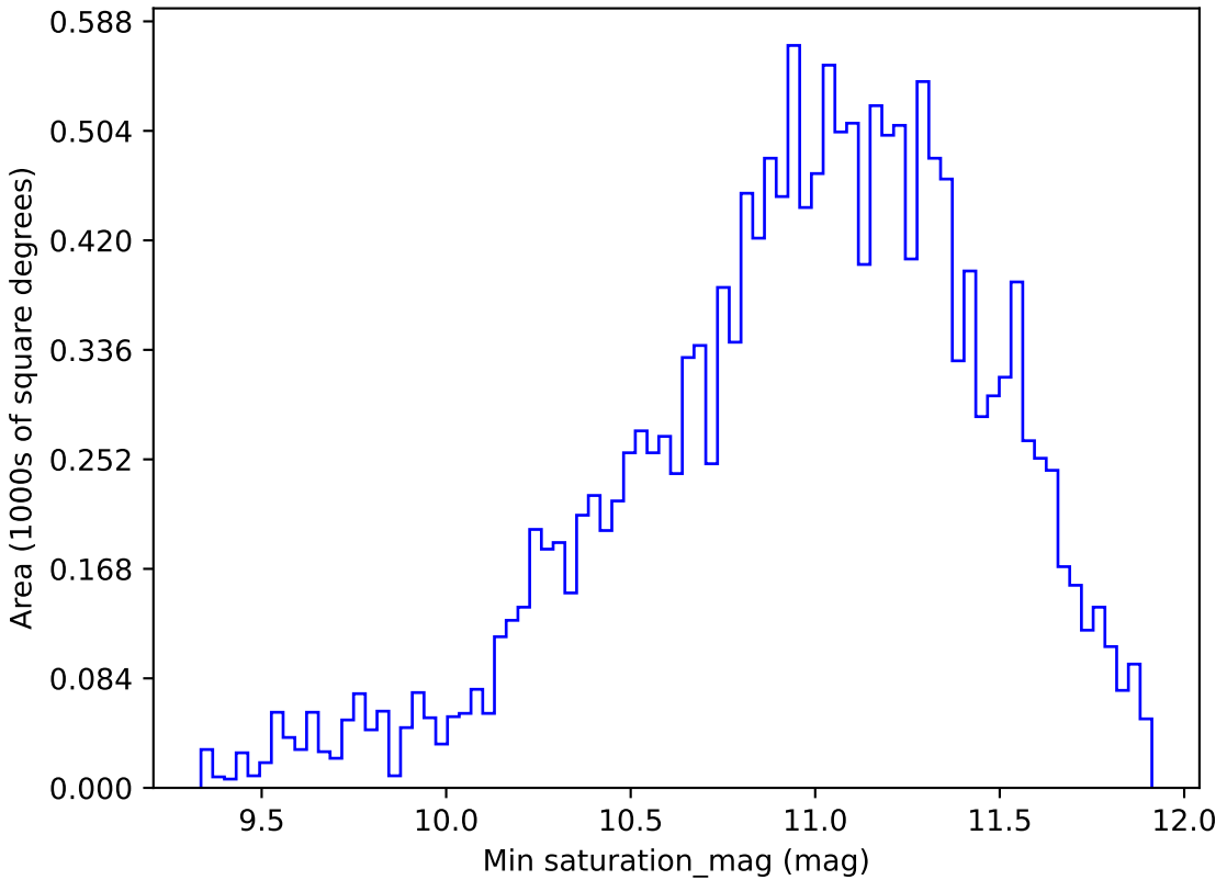
extra_ss_neo7_v3.4_10yrs WFD all bands: Min saturation_mag
