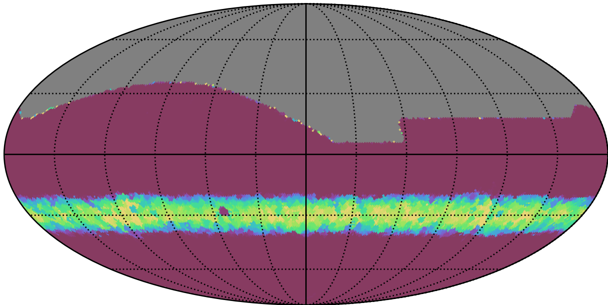
extra_ss_neo7_v3.4_10yrs All sky all bands: Min normairmass
