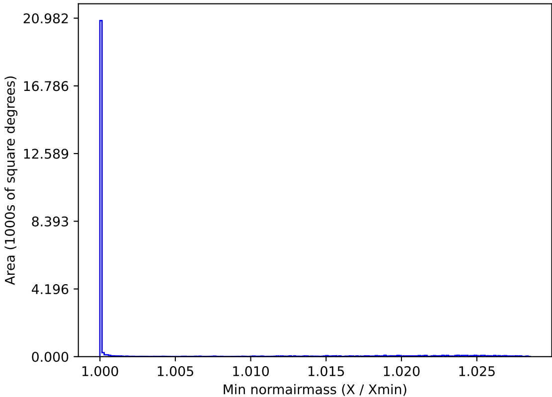
extra_ss_neo7_v3.4_10yrs All sky all bands: Min normairmass
