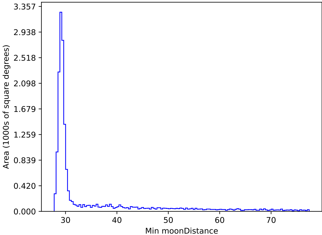
extra_ss_neo7_v3.4_10yrs WFD all bands: Min moonDistance
