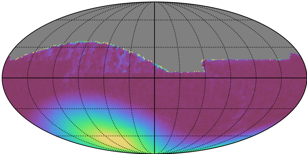
extra_ss_neo7_v3.4_10yrs All sky all bands: Min moonDistance
