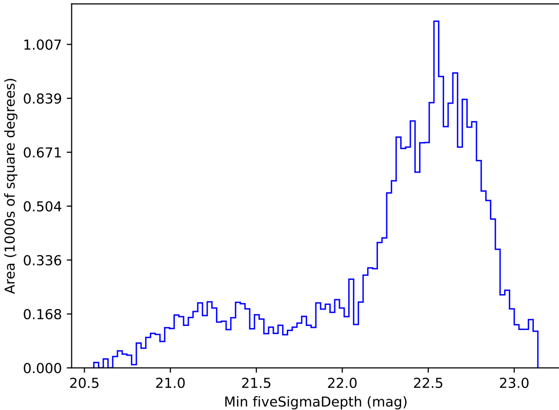
extra_ss_neo7_v3.4_10yrs Yr 1 z band: Min fiveSigmaDepth
