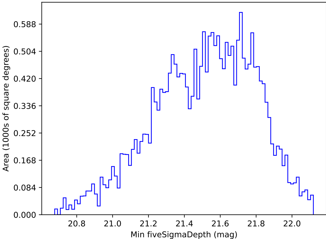
extra_ss_neo7_v3.4_10yrs Yr 1 y band: Min fiveSigmaDepth
