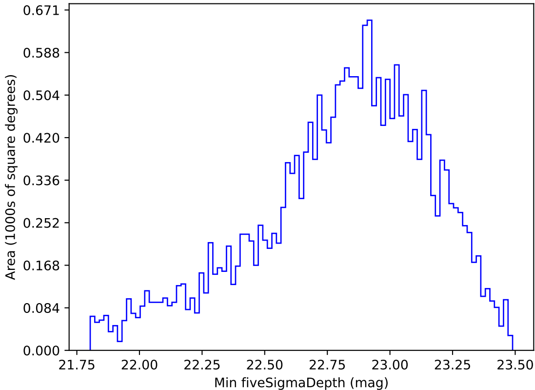
extra_ss_neo7_v3.4_10yrs Yr 1 u band: Min fiveSigmaDepth
