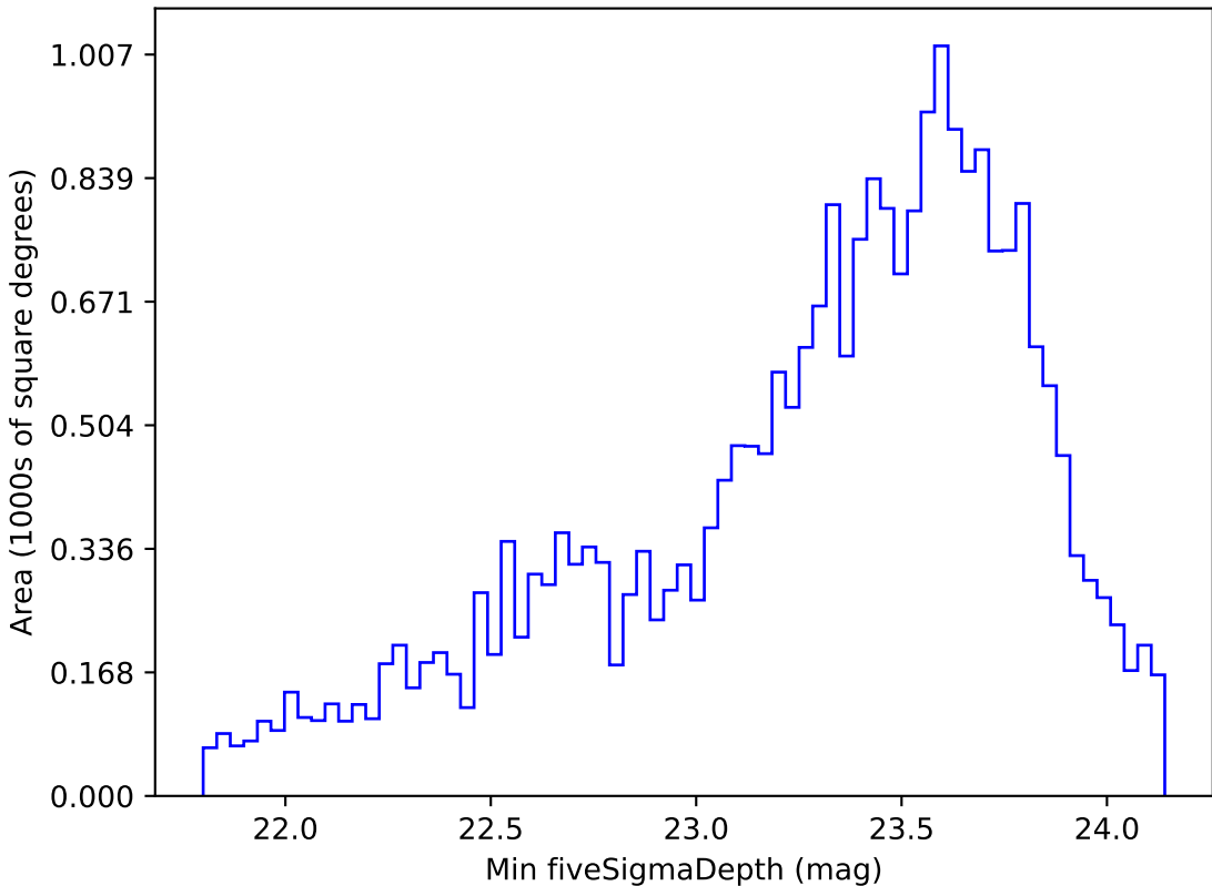
extra_ss_neo7_v3.4_10yrs Yr 1 r band: Min fiveSigmaDepth
