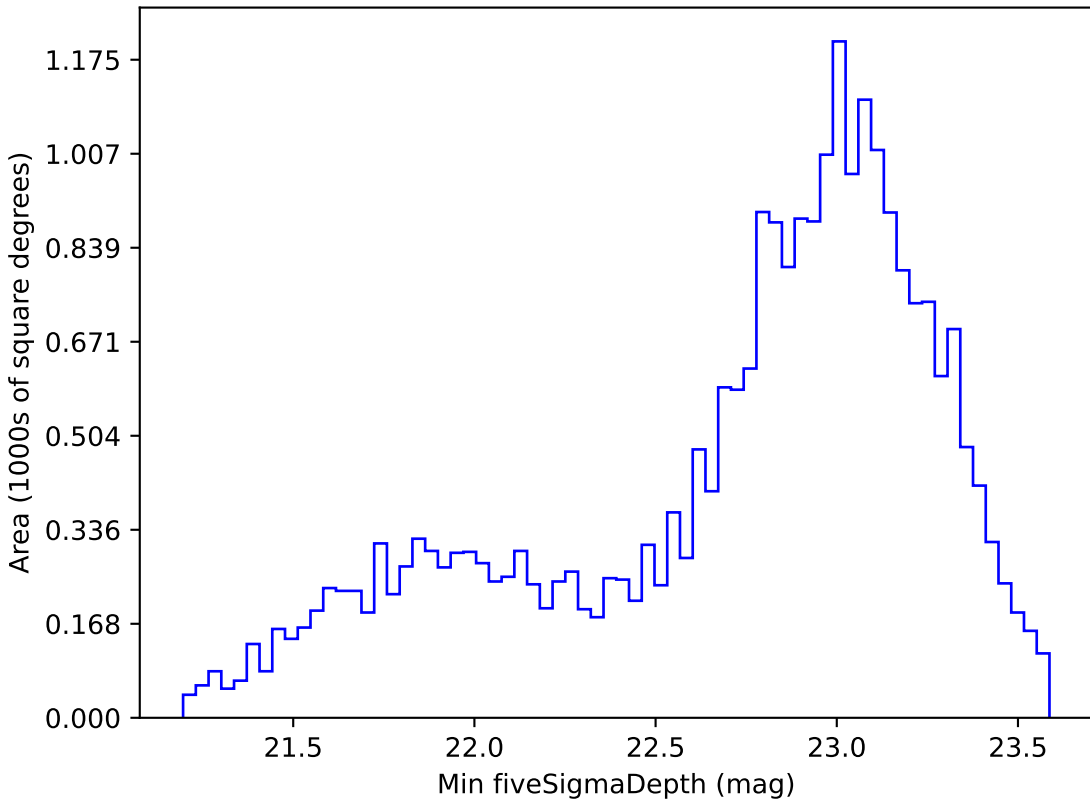
extra_ss_neo7_v3.4_10yrs Yr 1 i band: Min fiveSigmaDepth
