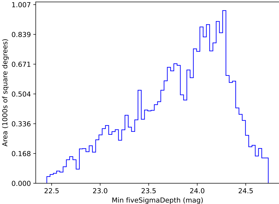
extra_ss_neo7_v3.4_10yrs Yr 1 g band: Min fiveSigmaDepth
