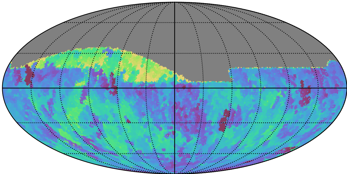
extra_ss_neo7_v3.4_10yrs Yr 1 all bands: Min fiveSigmaDepth
