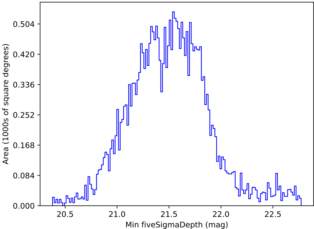
extra_ss_neo7_v3.4_10yrs Yr 1 all bands: Min fiveSigmaDepth
