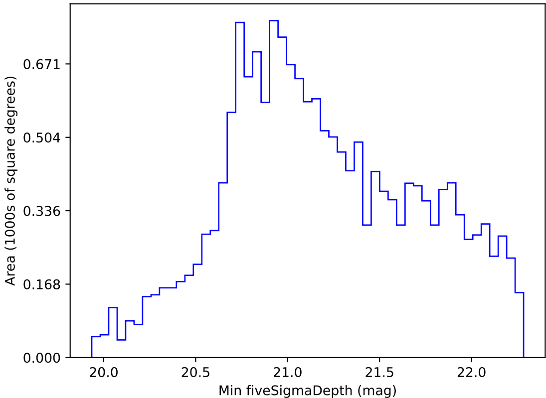
extra_ss_neo7_v3.4_10yrs WFD z band: Min fiveSigmaDepth
