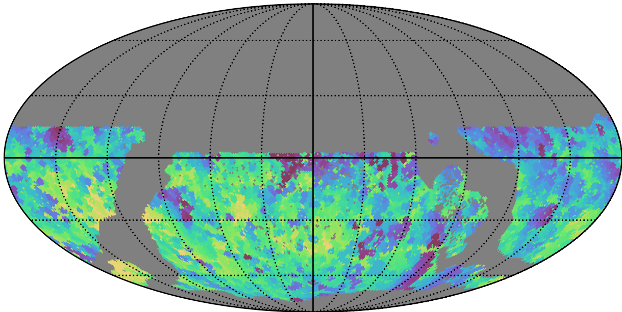
extra_ss_neo7_v3.4_10yrs WFD y band: Min fiveSigmaDepth
