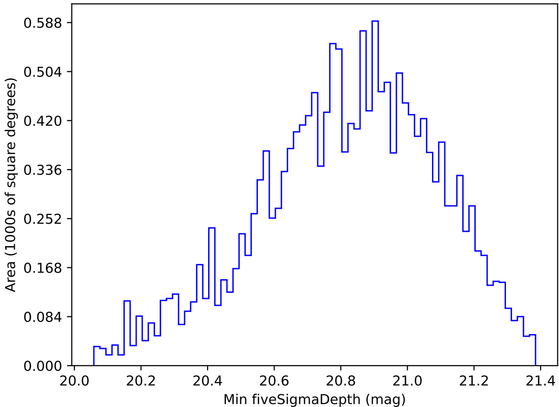
extra_ss_neo7_v3.4_10yrs WFD y band: Min fiveSigmaDepth
