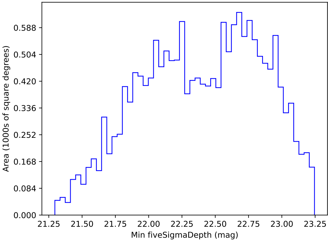
extra_ss_neo7_v3.4_10yrs WFD r band: Min fiveSigmaDepth
