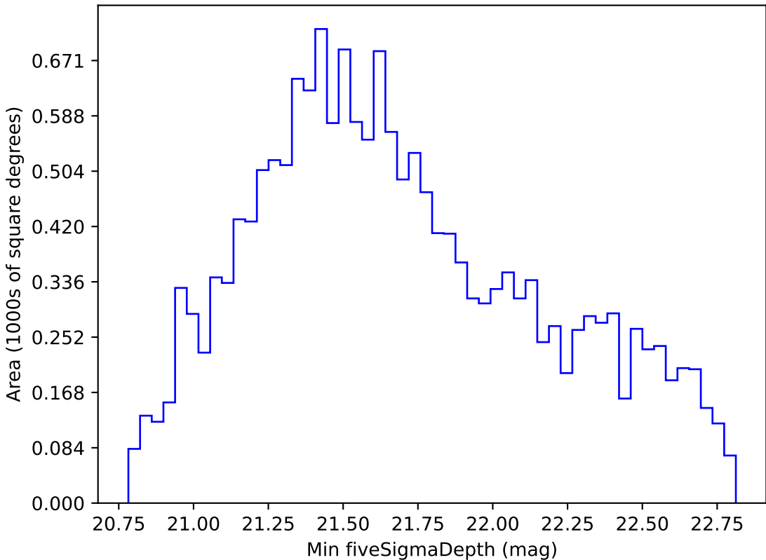
extra_ss_neo7_v3.4_10yrs WFD i band: Min fiveSigmaDepth
