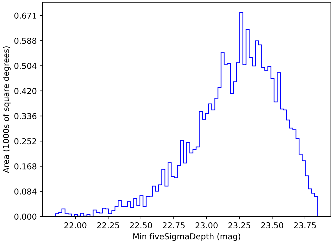
extra_ss_neo7_v3.4_10yrs WFD g band: Min fiveSigmaDepth
