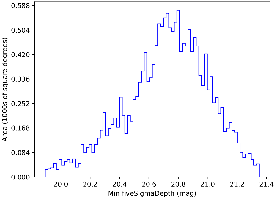
extra_ss_neo7_v3.4_10yrs WFD all bands: Min fiveSigmaDepth
