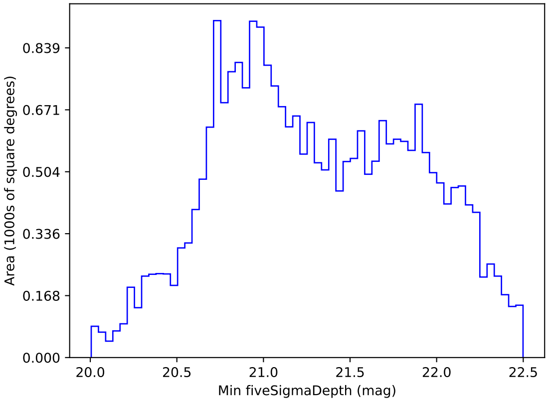
extra_ss_neo7_v3.4_10yrs All sky z band: Min fiveSigmaDepth
