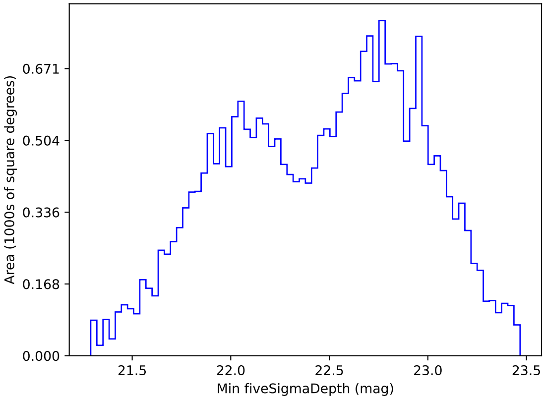
extra_ss_neo7_v3.4_10yrs All sky r band: Min fiveSigmaDepth
