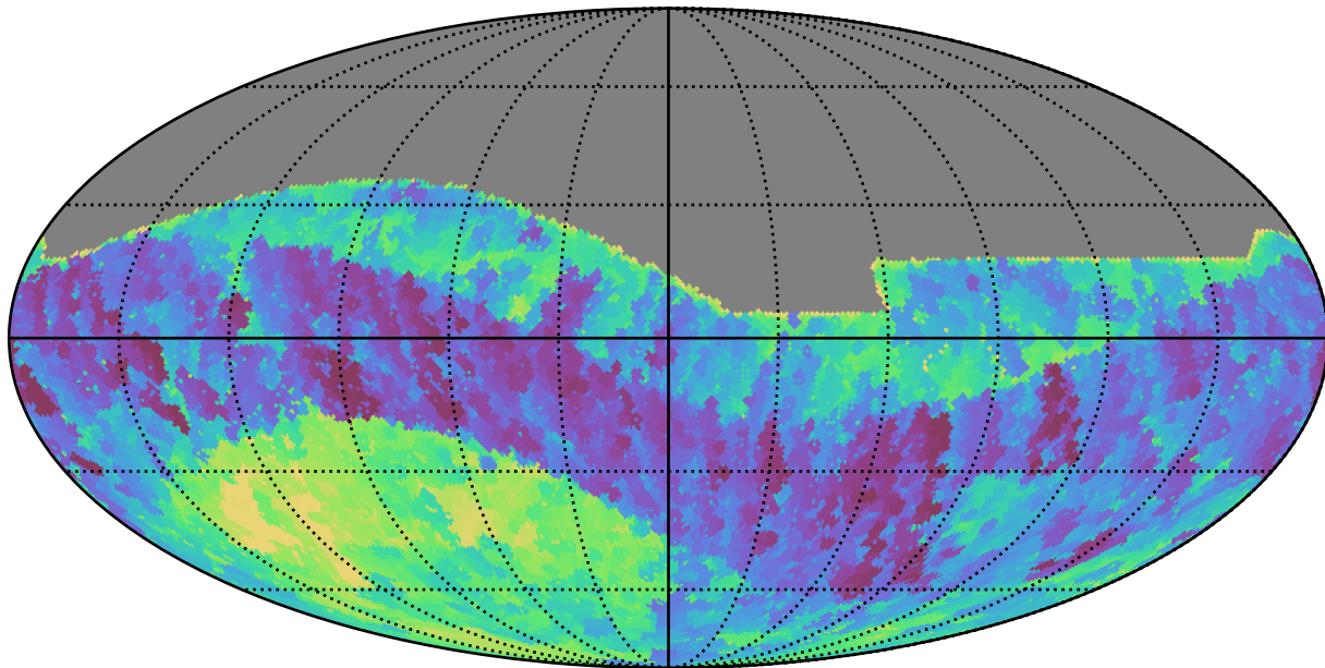
extra_ss_neo7_v3.4_10yrs All sky i band: Min fiveSigmaDepth
