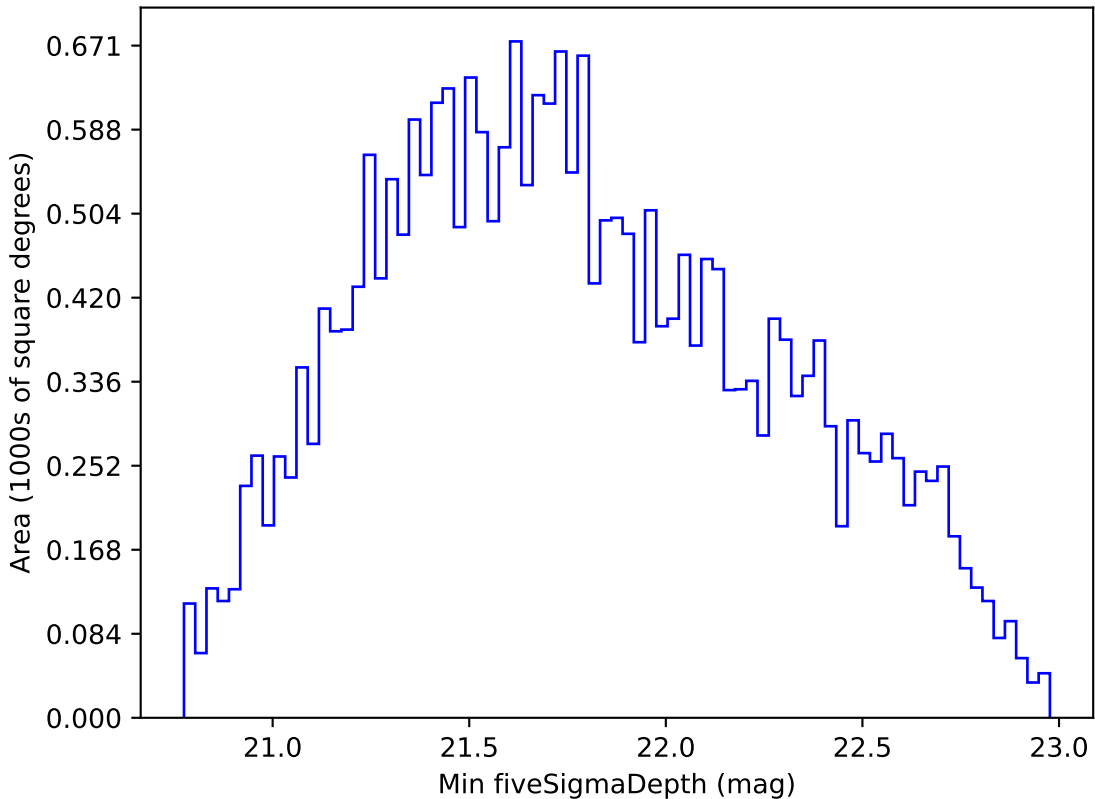
extra_ss_neo7_v3.4_10yrs All sky i band: Min fiveSigmaDepth
