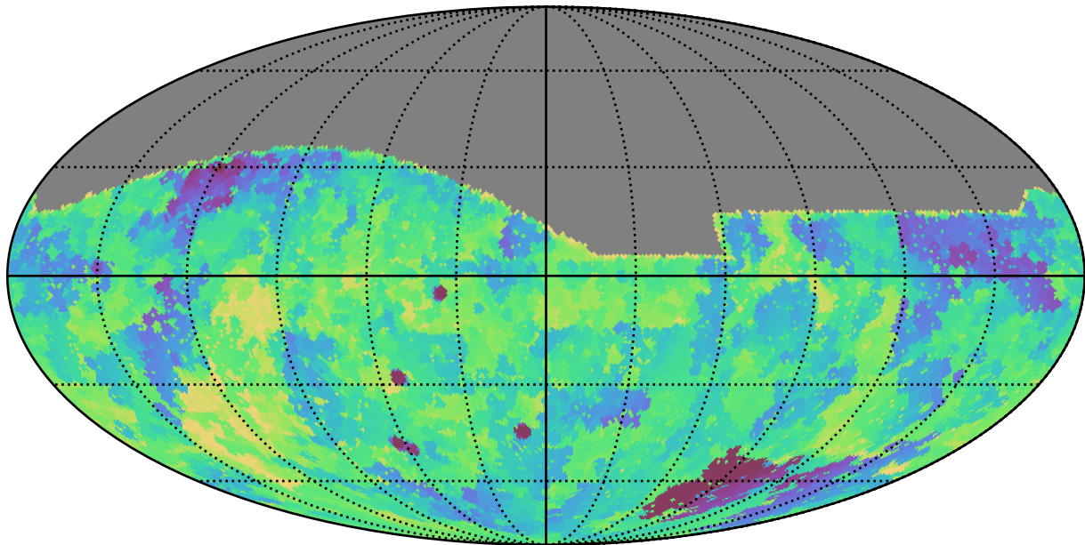
extra_ss_neo7_v3.4_10yrs All sky g band: Min fiveSigmaDepth
