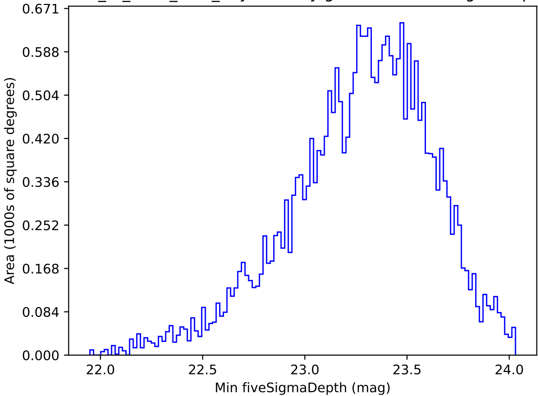
extra_ss_neo7_v3.4_10yrs All sky g band: Min fiveSigmaDepth
