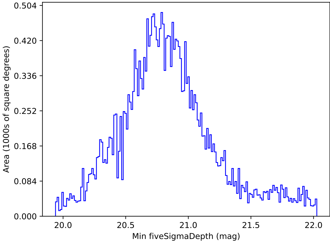
extra_ss_neo7_v3.4_10yrs All sky all bands: Min fiveSigmaDepth
