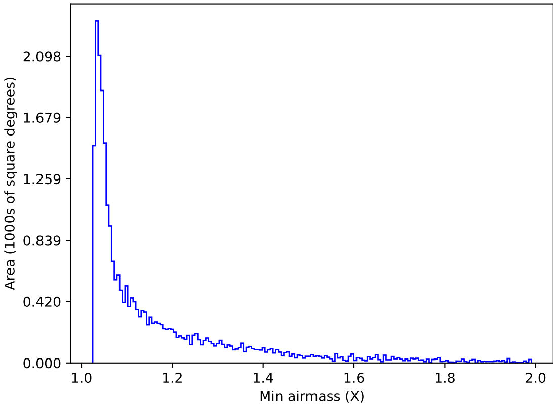
extra_ss_neo7_v3.4_10yrs Yr 1 z band: Min airmass
