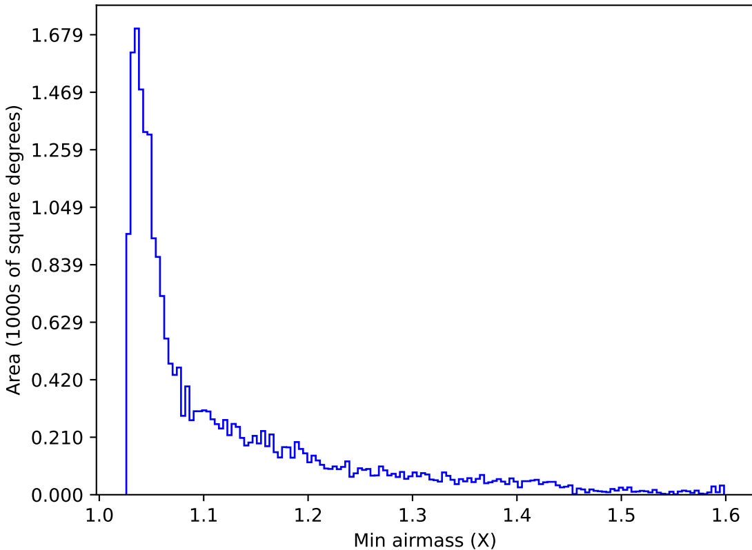
extra_ss_neo7_v3.4_10yrs Yr 1 y band: Min airmass
