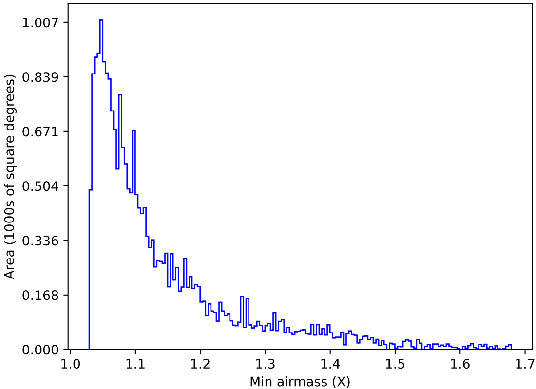
extra_ss_neo7_v3.4_10yrs Yr 1 u band: Min airmass
