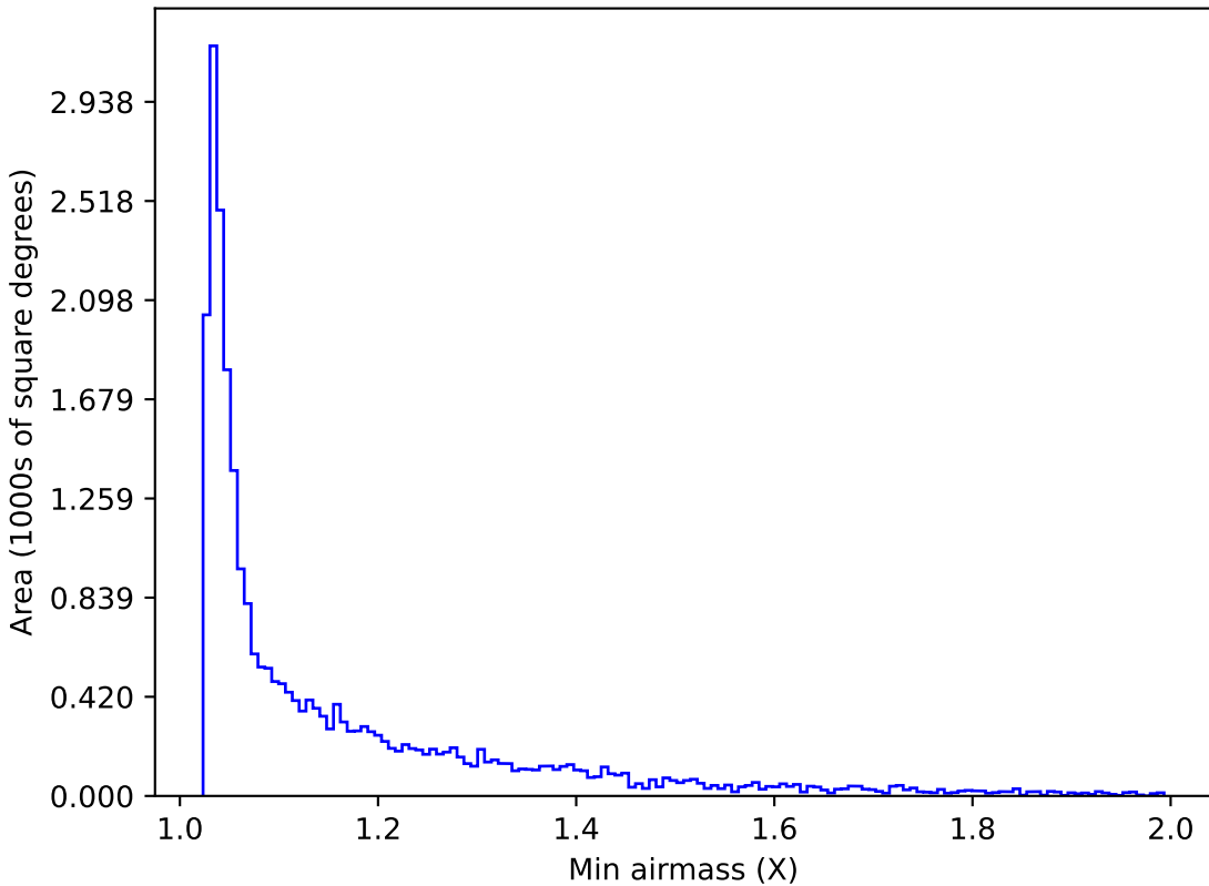
extra_ss_neo7_v3.4_10yrs Yr 1 i band: Min airmass
