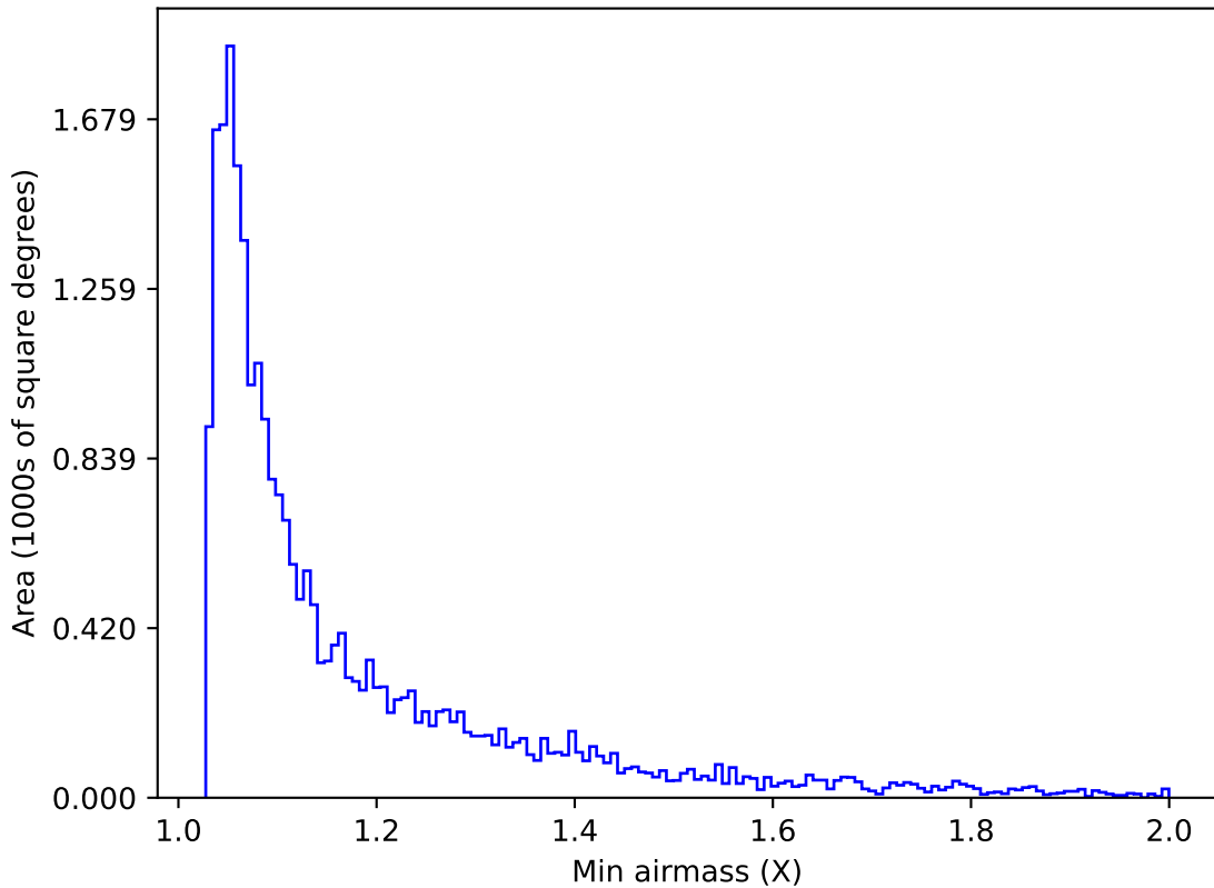
extra_ss_neo7_v3.4_10yrs Yr 1 g band: Min airmass
