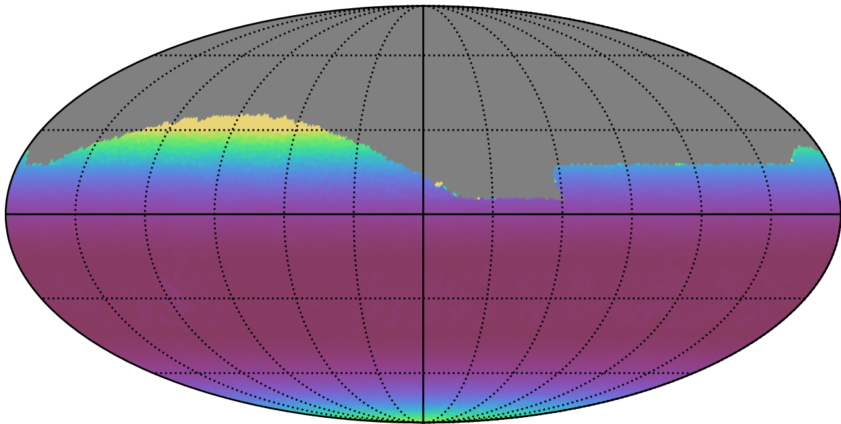
extra_ss_neo7_v3.4_10yrs Yr 1 all bands: Min airmass
