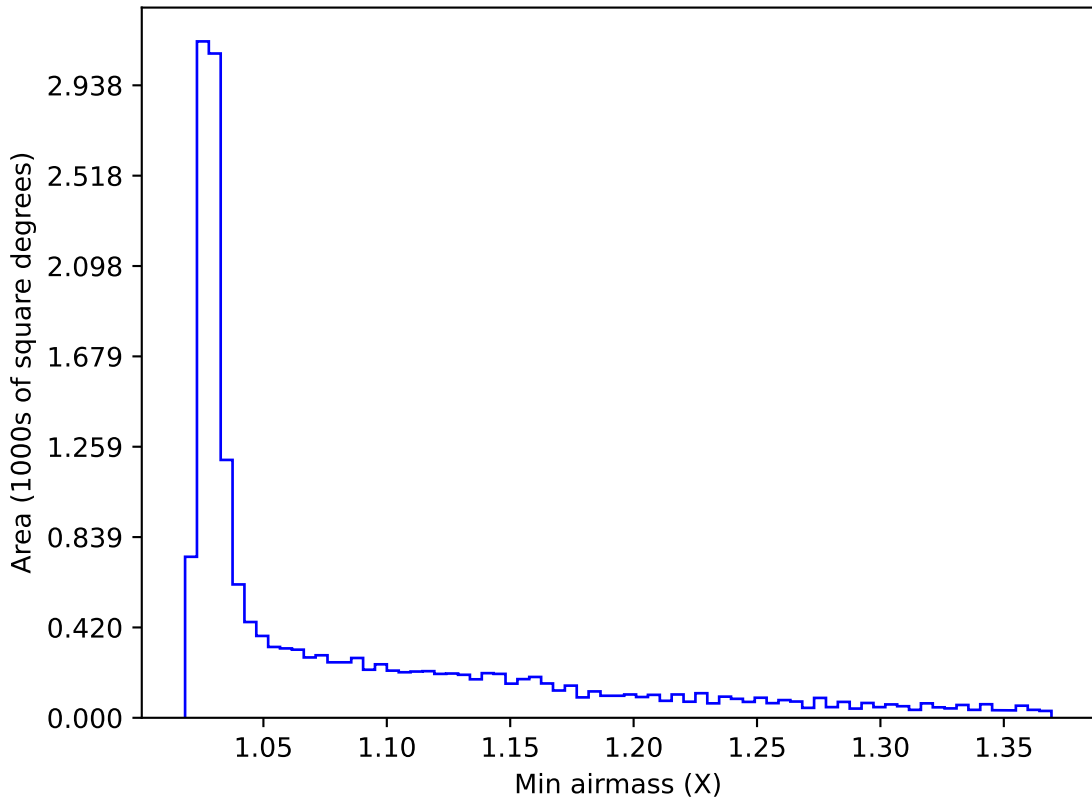
extra_ss_neo7_v3.4_10yrs WFD z band: Min airmass
