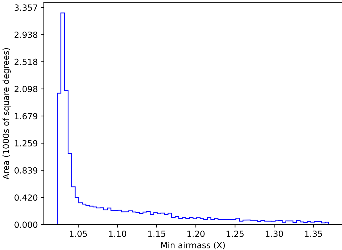
extra_ss_neo7_v3.4_10yrs WFD y band: Min airmass
