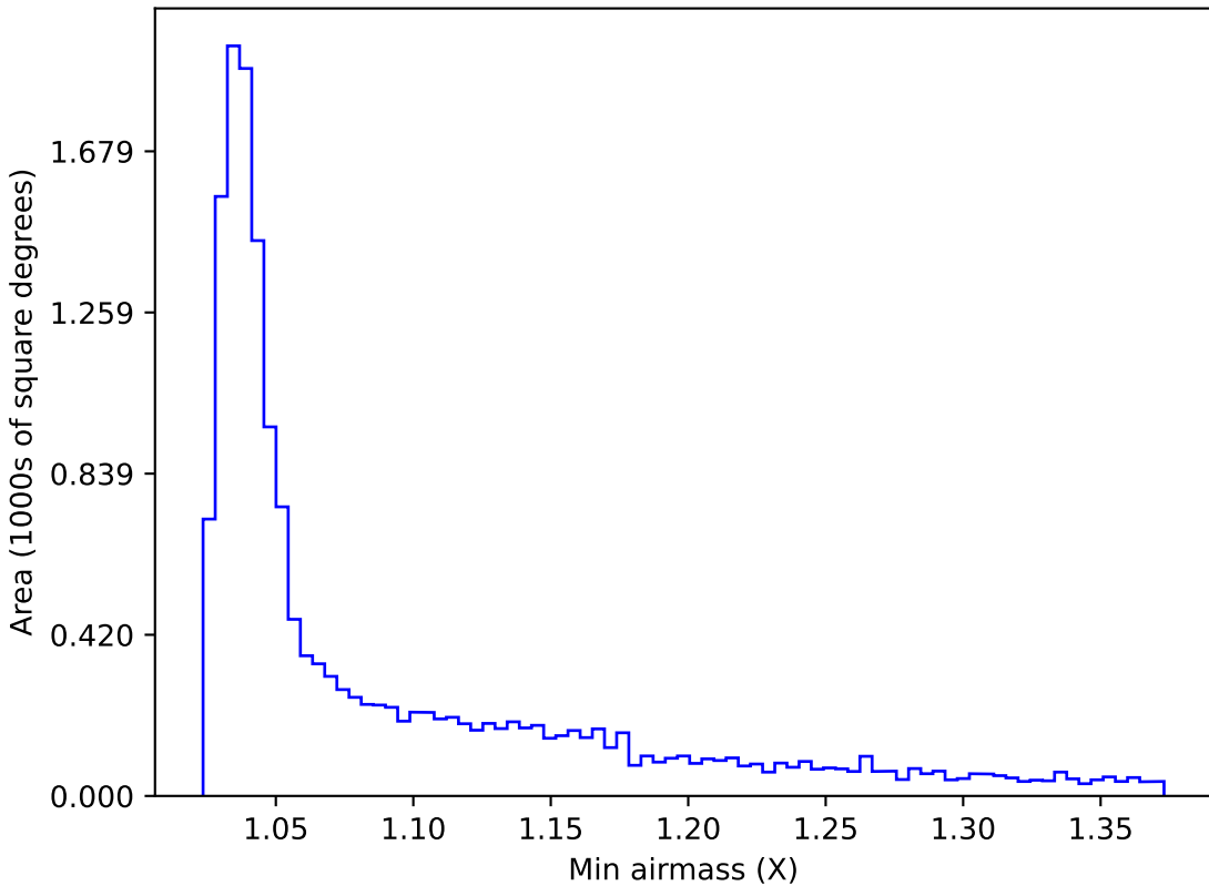
extra_ss_neo7_v3.4_10yrs WFD u band: Min airmass
