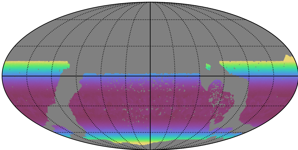
extra_ss_neo7_v3.4_10yrs WFD r band: Min airmass
