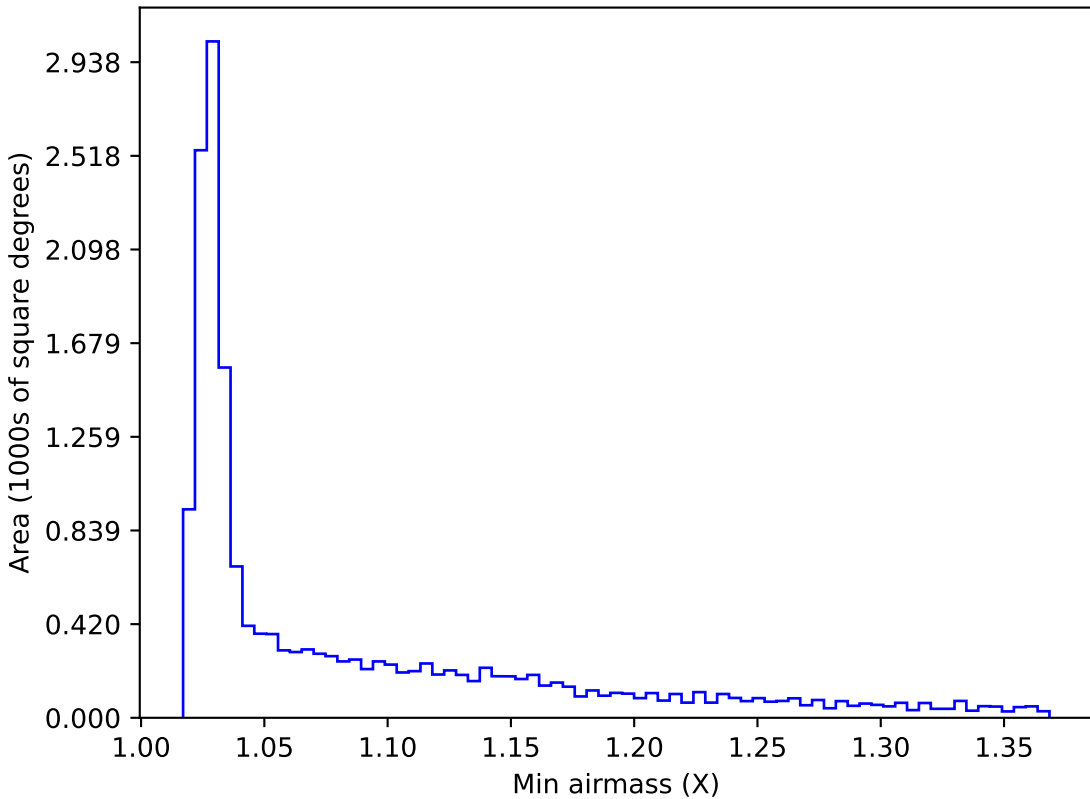
extra_ss_neo7_v3.4_10yrs WFD r band: Min airmass
